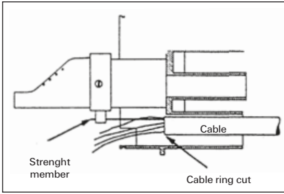
5.4 Align cable ring cuts with edge of base.
