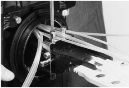
5.5 Install the screw and washer into the strength member fixation device. Slide the cable strength member under the washer and tighten the screw. Cut the excess length of the cable strength member.
