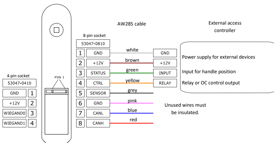
Connection diagram of the handle with the external access control system
