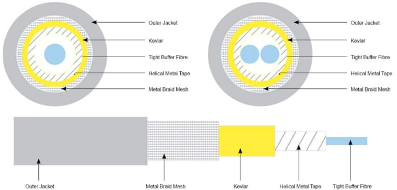
Simplex Patch cord Armoured
