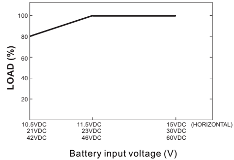
Figure 7.3: Input derating curve
