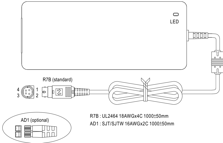
DC output connector (standard)
