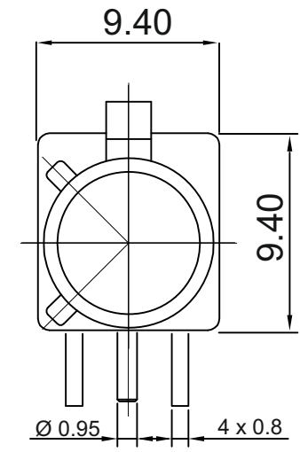
FAKRA D plug
