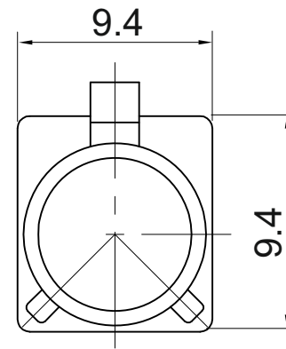
FAKRA K plug
