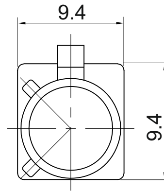
FAKRA D plug
