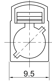
FAKRA C jack
