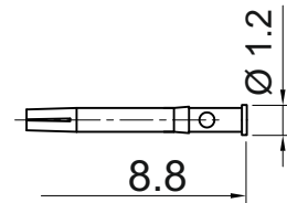
Pin contact
