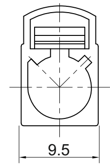
FAKRA B jack
