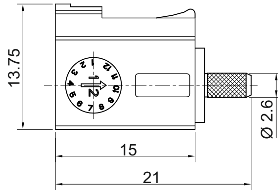
Plastic shell
