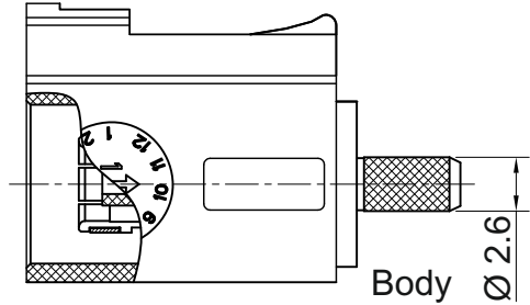
Plastic shell
