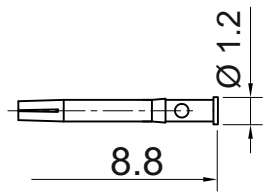
Pin contact
