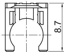
Snap ring
