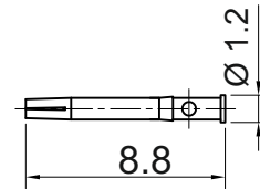
Pin contact
