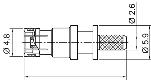
Body
