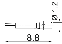
Pin contact
