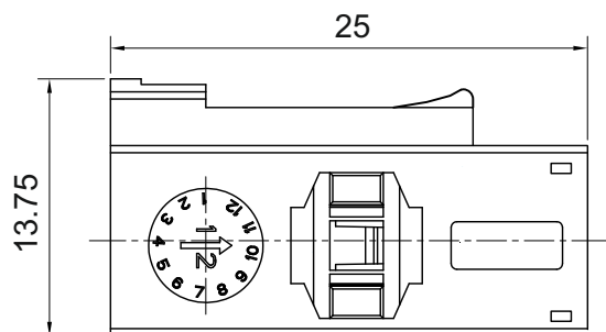
Plastic shell
