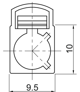
FAKRA D jack
