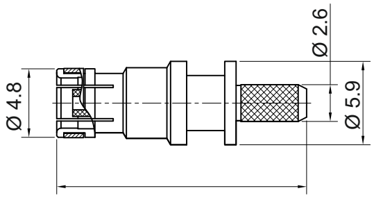
Body
