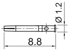
Pin contact
