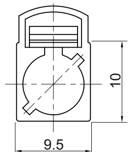
FAKRA C jack
