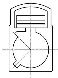
FAKRA F jack
