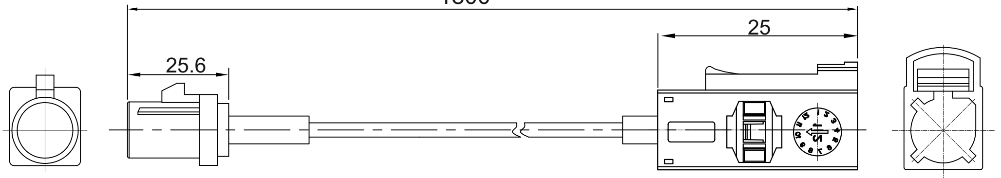
FAKRA Z plug
