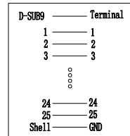
Pin assignment
